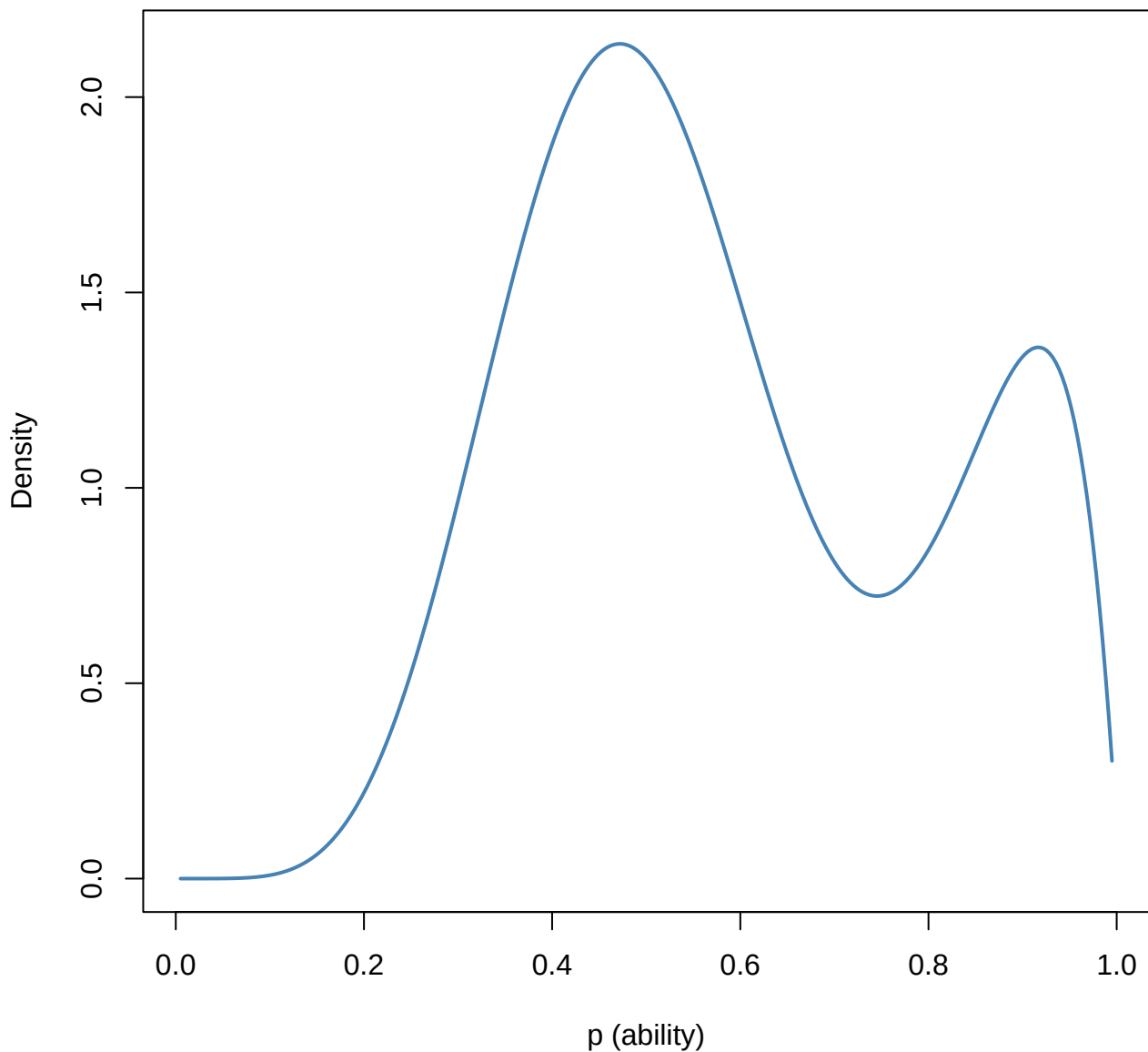
deAyala: estimated Bernstein prior density of p (K=13)
